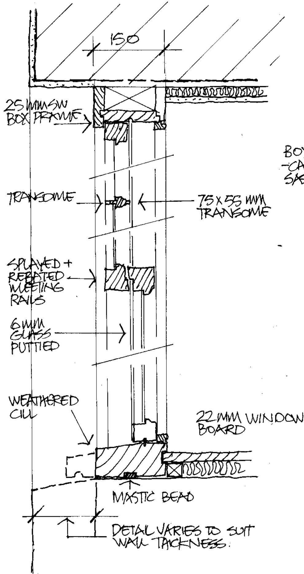
VERTICAL SECTION THROUGH BOX SASH.
